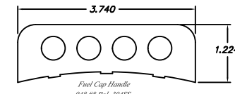
Fuel Cap Handle .048 #8 Pol. 304SS
